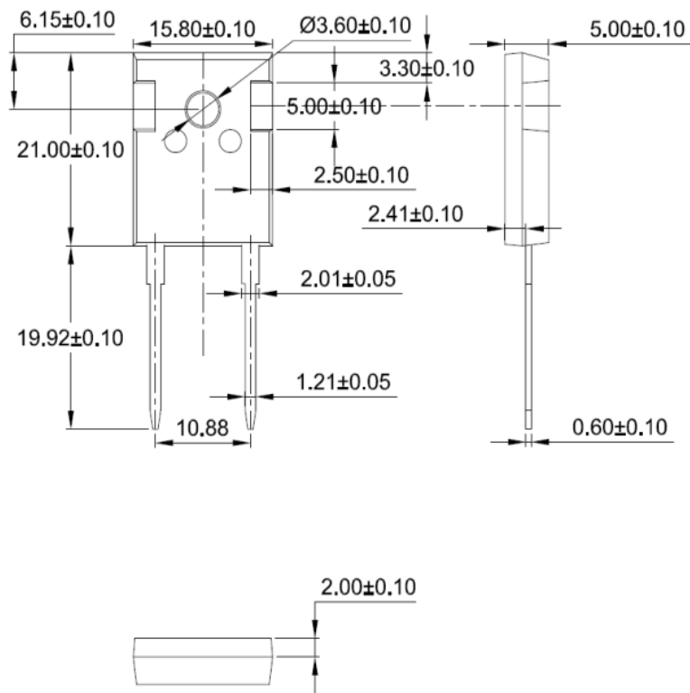
Figure 8. Package Outline
