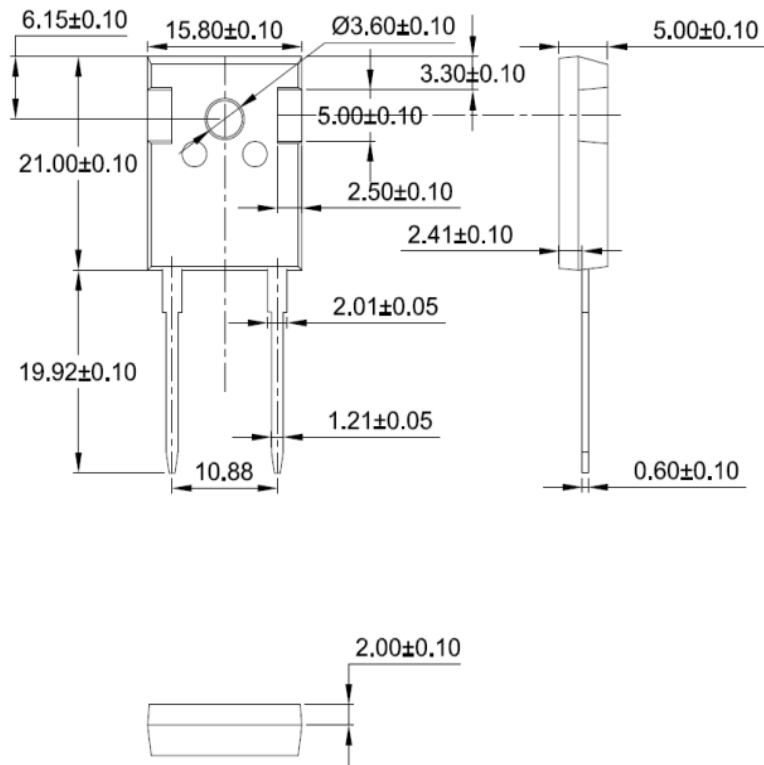
Figure 8. Package Outline
