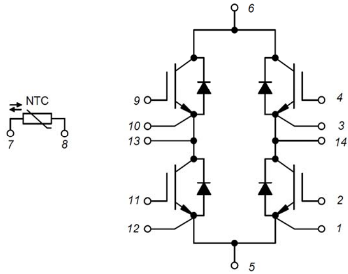
Figure 14. Circuit Diagram
