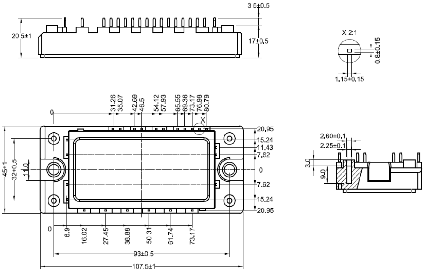
Dimensions in (mm) Figure 18. Package Outline
