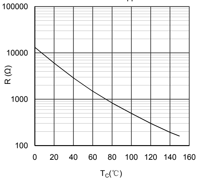
Figure 14. NTC Characteristics
