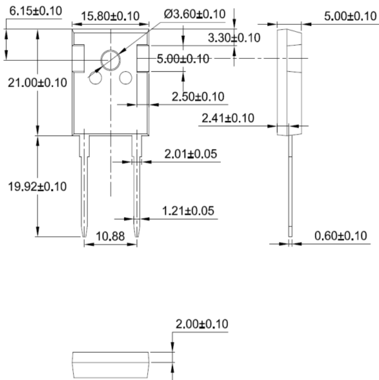
Figure 8. Package Outline
