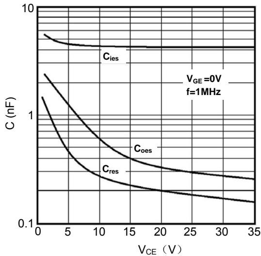
Figure8. Typical Capacitances vs. V_{CE}
