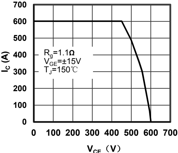
Figure 6. Reverse Biased Safe Operating Area
