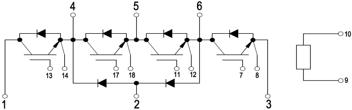
Figure 14. Circuit Diagram
