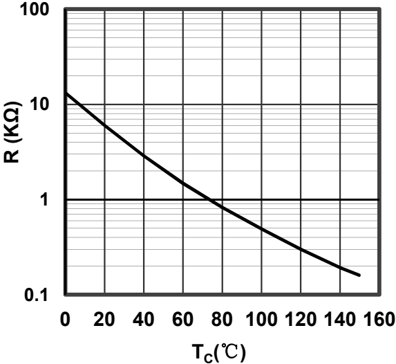
Figure 13. NTC Characteristics
