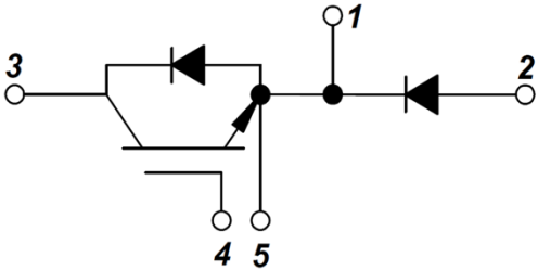
Figure 13. Circuit Diagram
