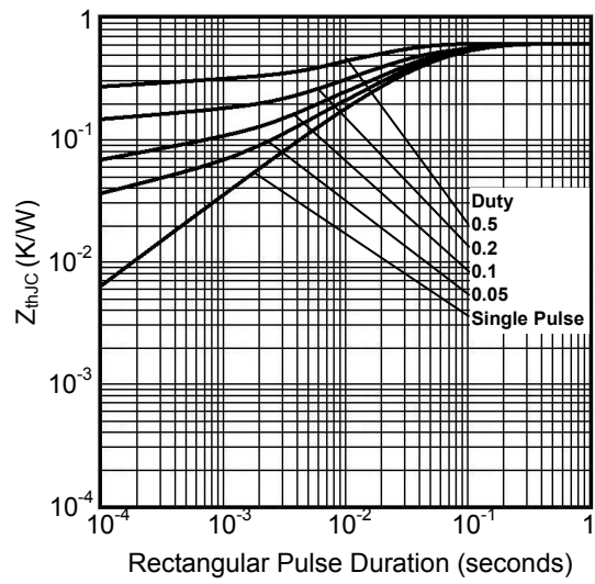
Figure14. Transient Thermal Impedance of Diode
