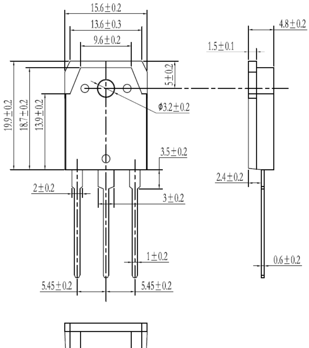
Dimensions in Millimeters Figure8. Package Outline
